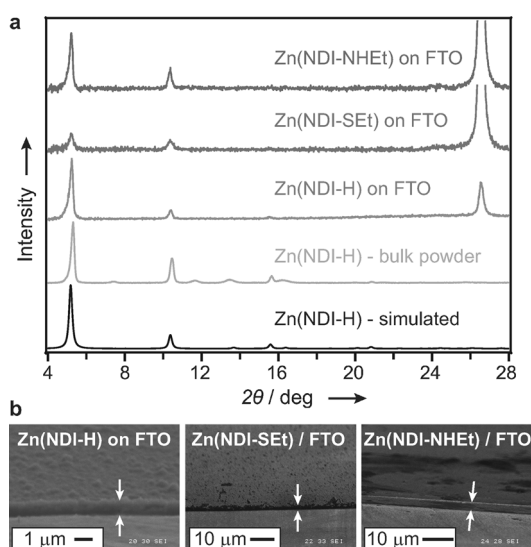
Figure 2. a) Powder X-ray diffraction patterns of \text{Zn}(\text{NDI-X}) ( \text{X} = \text{H}, \text{NHEt} , and \text{SEt} ) films on FTO substrates after washing (see the Supporting Information for details) and the bulk powder sample of \text{Zn}(\text{NDI-H}) for comparison. The prominent peak at 2\theta = 26.5^\circ corresponds to \text{SnO}_2 from the FTO substrate. b) Scanning electron micrographs of the \text{Zn}(\text{NDI-X}) films. White arrows indicate the surface of the MOF films and their contact with the FTO plate.
