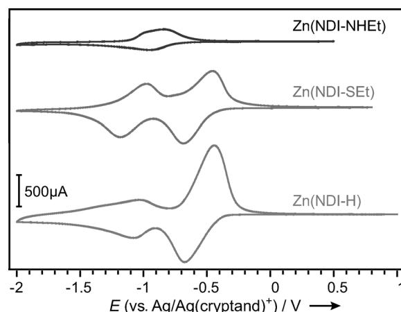
Figure 3. Cyclic voltammograms of \text{Zn}(\text{NDI-X}) ( \text{X} = \text{H}, \text{NHEt} , and \text{SEt} ) films on FTO substrates measured in DMF solution containing 0.1 M [(n\text{Bu})_4\text{N}]\text{PF}_6 at a scan rate of 50 \text{ mVs}^{-1} .
